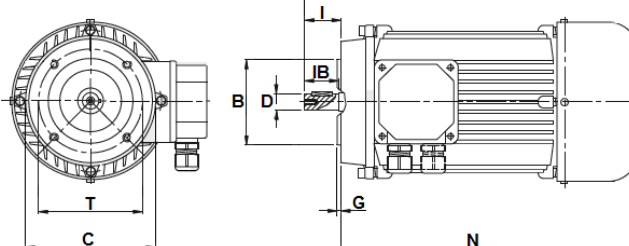
IEC - B14
