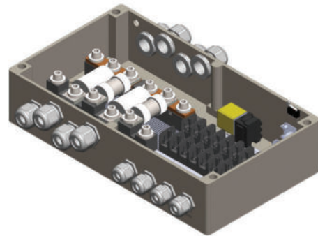
Power Distribution Unit for Electric Vehicles
