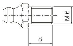
DIN 71412, cone-type nipple for carriage size 25, 30, 35 and 45
