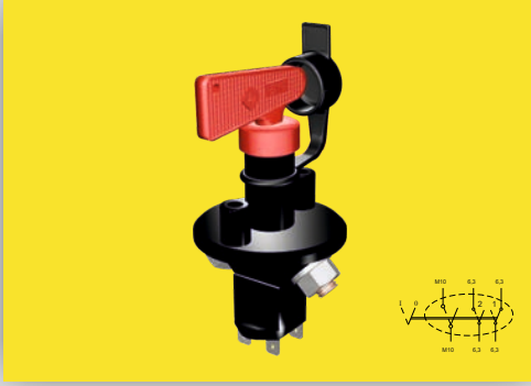
05 0308 DEVRE KESİCİ KORUMALI BATTERY CUT - OFF SWITCH
