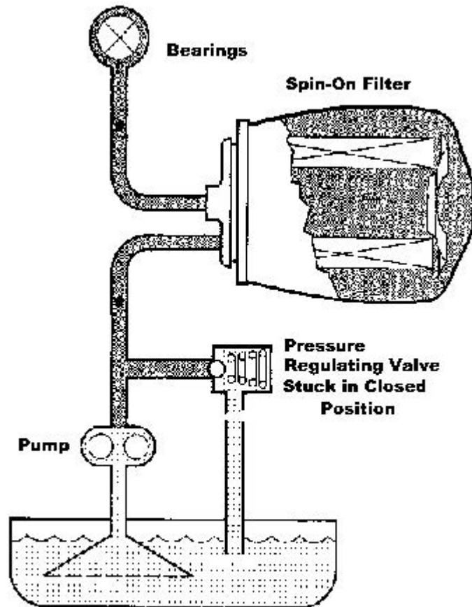
EXCESSIVE PRESSURE FIG. 2
