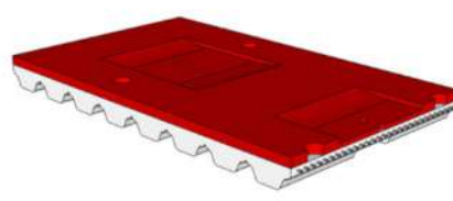
Longitudinal milling with tooth removal and complex machining
